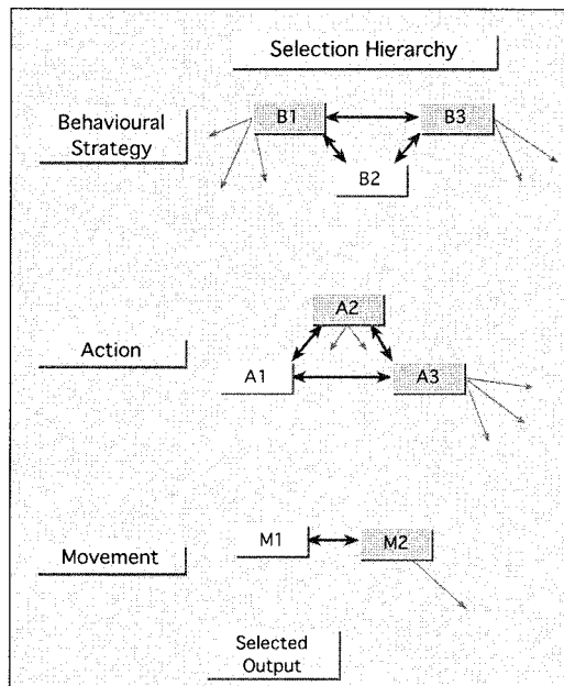
Fig. 2. Hierarchical decomposition of the selection problem. Again, levels of activity within different components are represented by density of shading; light=high activity. The dark arrows at each level represent reciprocal inhibitory connections which would support ‘winner-take-all’ selection between elements. Selections at the highest level determine overall behavioural objective (B1–3). Activated connections (white arrows) from the selected/winning element (B2) represent priming signals to lower level components associated with that element. Grey arrows represent non-activated priming signals from non-selected/losing elements. At intermediate levels, action (A1–3) which can achieve higher level objectives is selected (A1). At the lowest levels (M1–2) selection enables a pattern of motor activity (M1) which can produce the selected action.
