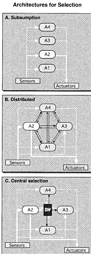
Fig. 3. Architectures proposed to solve the selection problem. (A) A hierarchical 'subsumption' architecture 8 in which disputes between actions (A1–4) represented in different layers are resolved by a pre-programmed fixed priority scheme. (B) A 'distributed' network in which each competing module (A1–4) has a reciprocal inhibitory connection with every other and an excitatory link to the shared output resource. Solid white arrows represent greater support for A2 which in turn imposes greater reciprocal inhibition on competing elements (black vs grey arrows). (C) A central selection mechanism can be used to determine access to the shared output resource with fewer connections. Note the central switch (SW) detects greater support for element A2 and provides return facilitation for this element (white arrows); less well supported ('losing') elements are inhibited (dark arrows) by the central switch.
